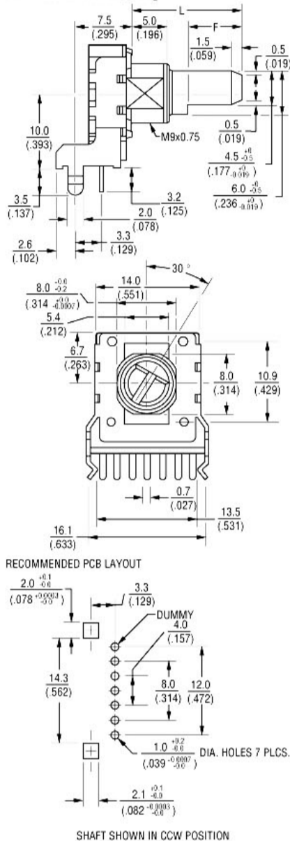
PTV142B-2 With Bushing
