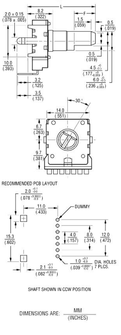
PTV142B-4 No Bushing
