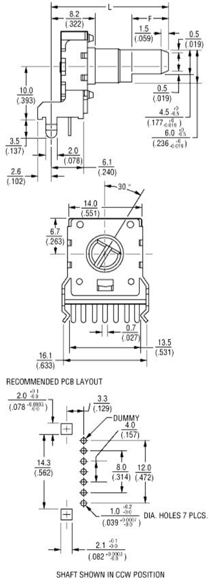
PTV142B-2 No Bushing
